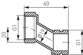
mounting GM without eccentrics
