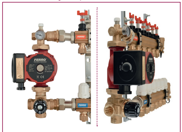
mounting GM by means of eccentrics
