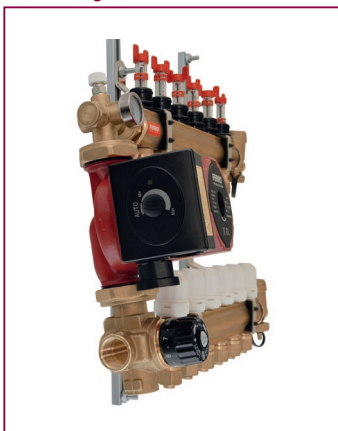
mounting GM without eccentrics
